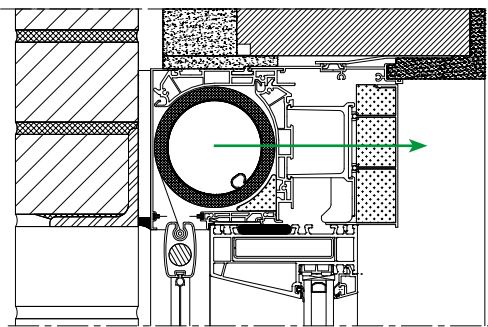
Montagesituatie 4: Fixscreen® Mono AK Large+
