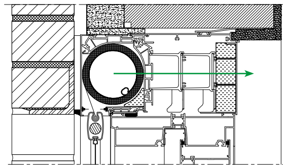
Montagesituatie 4: Fixscreen® Mono AK X-Large+
