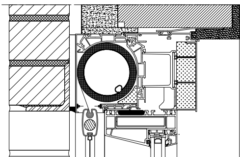
Fixscreen® Mono AK Large+
