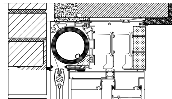
Fixscreen® Mono AK X-Large+
